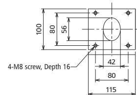
Hopper base
