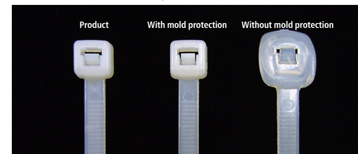
Comparison of cable tie crushing with/without mold protection
