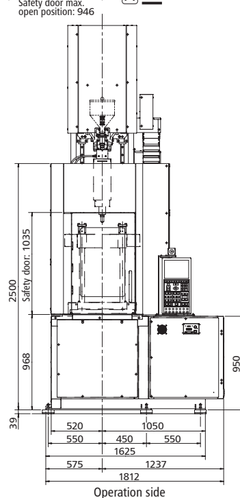
Operation side
