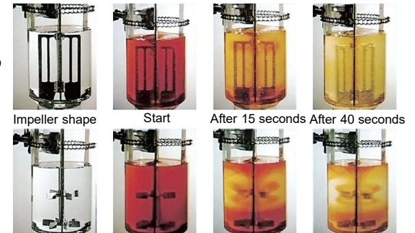
Comparison of mixing times using the iodine decolorization reaction (where the liquid becomes transparent as mixing progresses)
